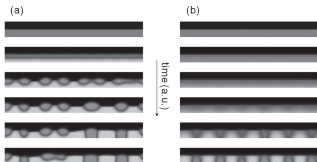
Figure 3. Evolution of blend topography with time. Simulated cross sections of blend films are presented as a function of time (the time increases from top to bottom): a) simulation at low temperature by taking \chi_{\text{PFO-P(VDF-TrFE)}} = 0.6 and b) simulation at high temperature by taking \chi_{\text{PFO-P(VDF-TrFE)}} = 0.4 .
